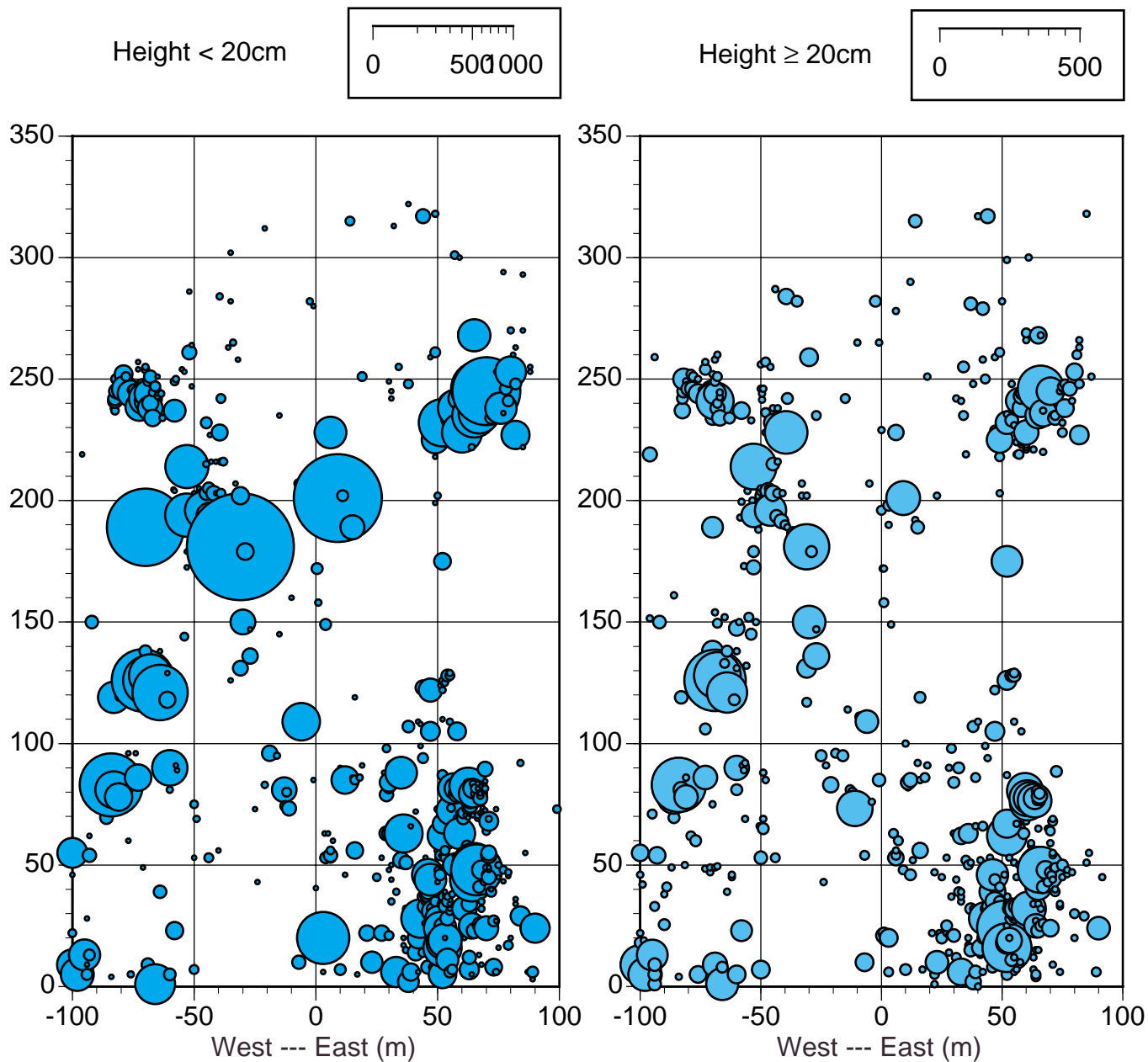
The coordinate (0,0) corresponds to the pole G12. The diameter of a bubble indicates the number of stems per square meter for each size class.
